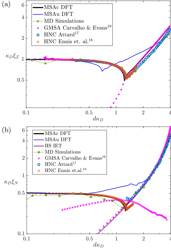
FIG. 6. The decay lengths obtained from different theories are compared with simulation results for the bulk decay lengths (green dots). In (a) the Z decay length obtained from our DFT calculations of one-body profiles (solid lines) are shown along with the bulk decay lengths obtained using the GMSA from Carvalho & Evans Ref. 19 (purple asterisks), the HNC from Attard 17 (blue circles) and the HNC from Ennis et al. 18 (orange squares). In (b) the N decay length from the same sources, but also including the result from the HS IET (solid purple line).
