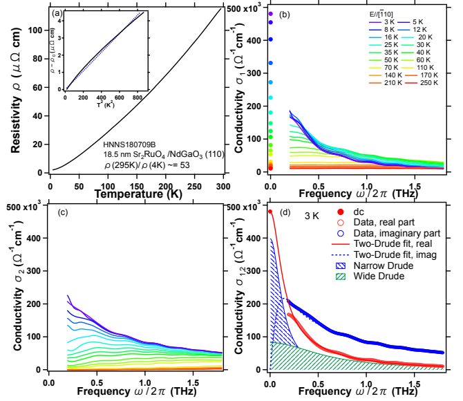
FIG. 6. (color online) (a) dc resistivity as a function of temperature for the Sr 2 RuO 4 film. The data is a geometric mean of the [110] and [001] directions of the NdGaO 3 substrate. Inset: Resistivity minus residual resistivity as a function of temperature squared. Fits to the data in the temperature range 2-32 K is shown as black lines. (b) Real and (c) imaginary parts of the THz conductivity \sigma_{1,2} from 3 K to 250 K. The markers at zero frequency are dc conductivity. (d) Two Drude fit of dc plus THz data at 3 K. dc conductivity, real and imaginary parts of the optical conductivity are fitted simultaneously. For all THz data, E//[110] .
