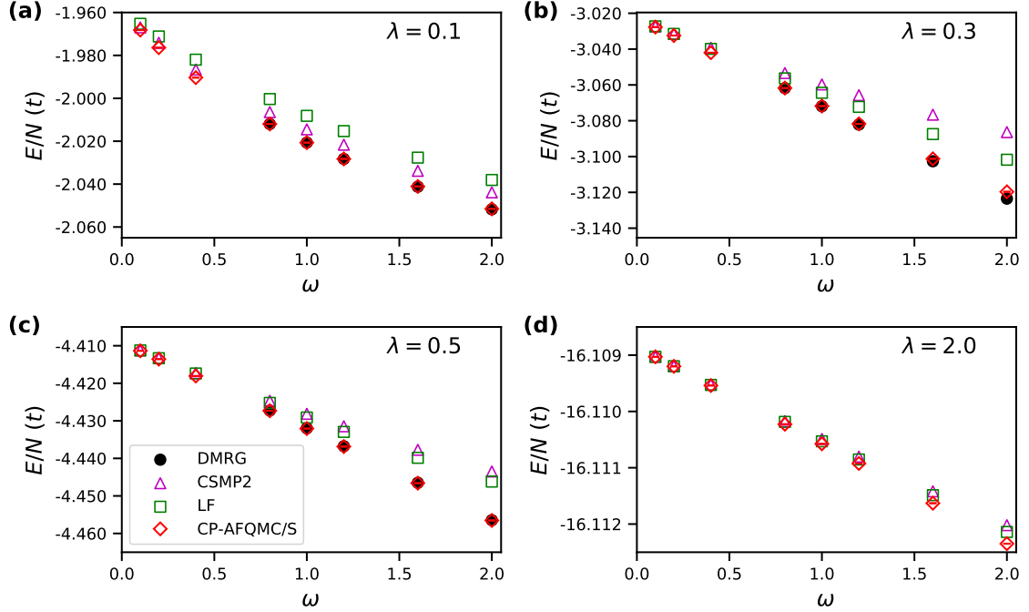
FIG. 4. Total energy per site in units of t for the 4x4 2D Holstein model at half-filling as a function of \omega for various \lambda values: (a) \lambda = 0.1 results, (b) \lambda = 0.3 results, (c) \lambda = 0.5 results, and (d) \lambda = 2.0 results. Note that all error bars of CP-AFQMC/S are too small to be seen on the plotted scales, DMRG reference values are only available for \omega \geq 0.8 when \lambda < 2.0 .
