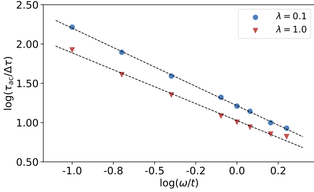
FIG. 5. Log-log plot of autocorrelation time \tau_{ac}/\Delta\tau and phonon frequency \omega/t for \lambda = 0.1 and \lambda = 1.0 . The black dotted lines are linear fits for each curve. For \lambda = 0.1 , the slope is -0.9876 with R^2 = 0.9993 and for \lambda = 1.0 , the slope is -0.8617 with R^2 = 0.9942 .
