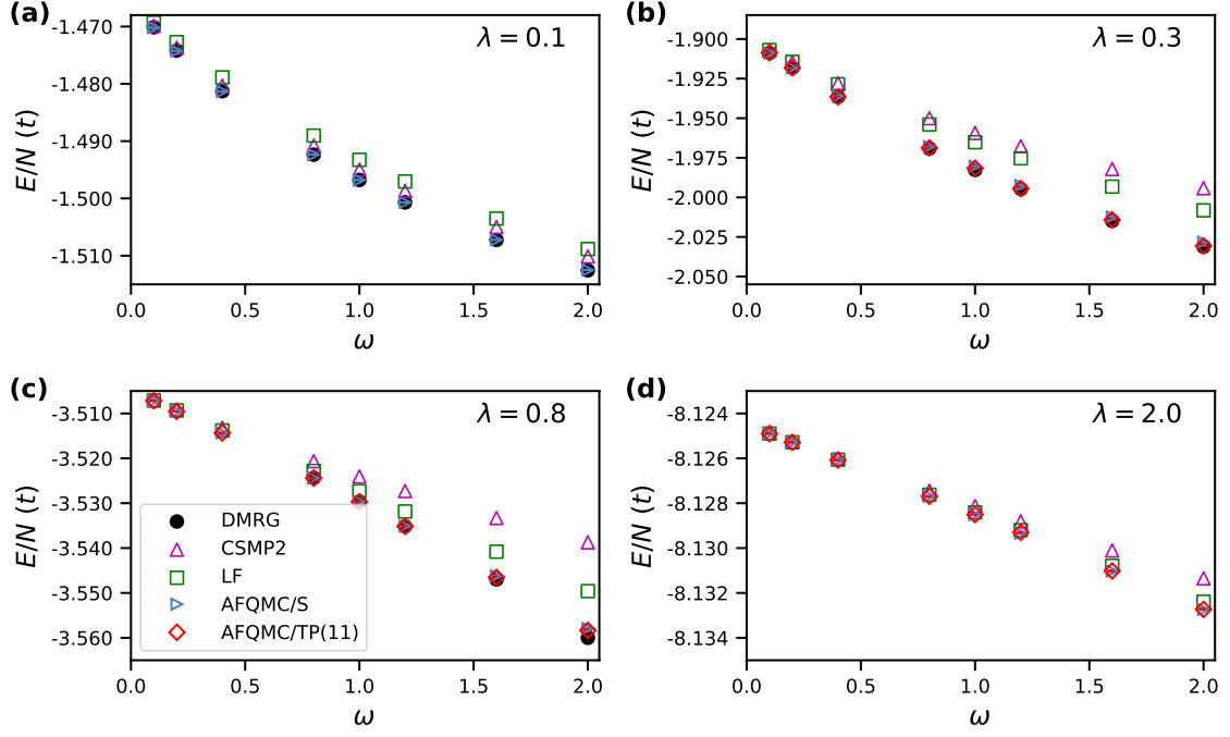
FIG. 3. Total energy per site in units of t for the 20-site 20-electron 1D Holstein model as a function of \omega for various values of \lambda values: (a) \lambda = 0.1 results, (b) \lambda = 0.3 results, (c) \lambda = 0.8 results, and (d) \lambda = 2.0 results. Note that all error bars for AFQMC are too small to be seen on the plotted scales, DMRG reference values are unavailable for \omega < 0.8 when \lambda = 0.8 and \lambda = 2.0 , and AFQMC/TP(11) is not presented for \lambda = 0.1 because the results for this trial wavefunction are nearly identical to those of AFQMC/S.
