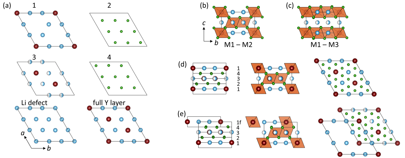
Figure 3: Construction of stacking fault models. (a) individual layers. Atom legend: red for Y; blue for Li; green for Cl. Side on view of the (b) M1 - M2 and (c) M1 - M3 models proposed by Schlem et al. 55 (d) M1 - M2 layered model that serves as the starting point for the stacking fault model construction (e) illustration of the (1/3, 2/3) layer 1 fault that is responsible for the majority change in the X-ray diffraction pattern. One notes that the \text{Li}^+ substructure is essentially unchanged by this fault and the major consequence is the creation of face sharing Y-Cl species along the center of the unit cell.
