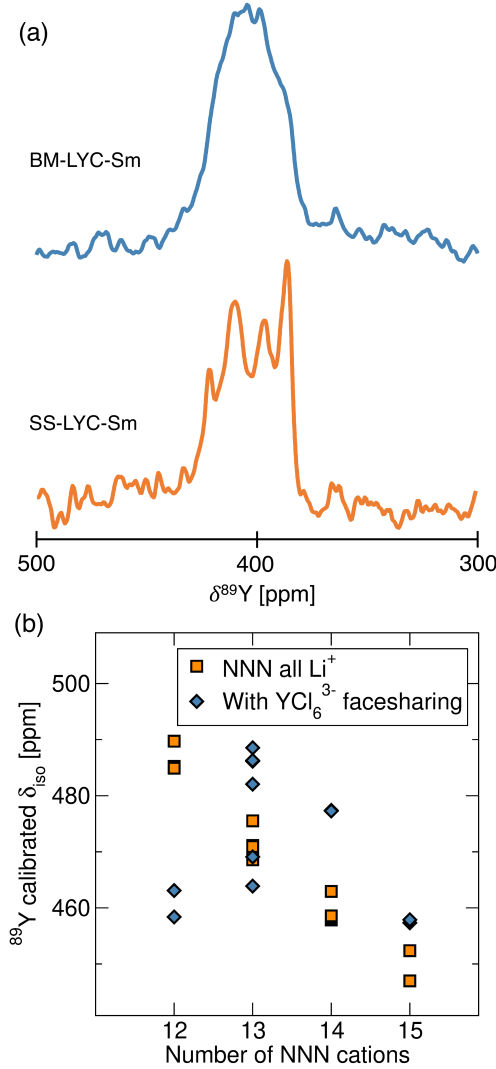
Figure 7: (a) ^{89}\text{Y} resonances for the Sm-doped LYC samples, BM-LYC-Sm and SS-LYC-Sm. All spectra were acquired at 18.8 T and a 10 kHz MAS rate with a set temperature of 298 K. (b) Isotropic ^{89}\text{Y} chemical shifts plotted as a function of the number of next nearest neighbor ( NNN ) cations for each corresponding \text{Y}^{3+} . The shifts were computed with DFT for bulk orderings within 25.5 \text{ meV atom}^{-1} from the convex hull in Figure 5.
