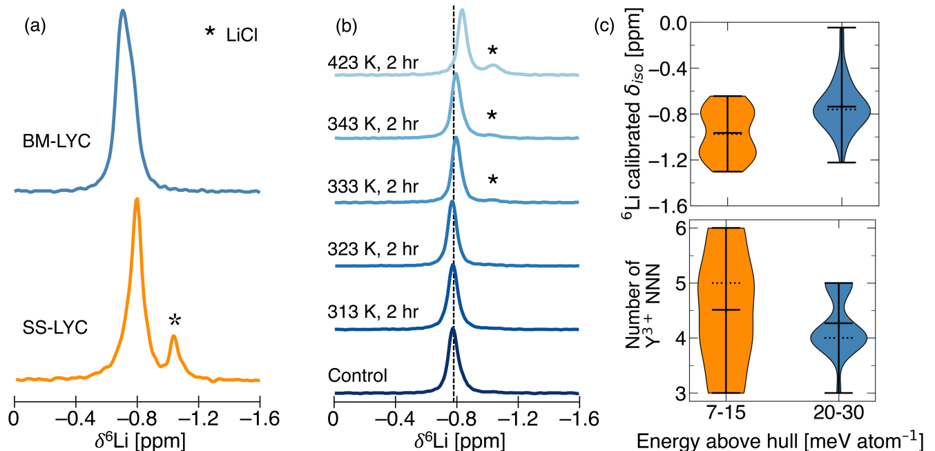
Figure 6: (a) {}^6\text{Li} NMR spectra for as-prepared BM-LYC and SS-LYC. (b) {}^6\text{Li} NMR spectra collected on a series of BM-LYC samples heat treated at various temperatures from room temperature to 423 K (150°C). Besides the control sample which was only sealed in a capillary, all samples were heated in a sealed capillary for a period of \approx 2 hours. LiCl is labeled with an asterisk (*). All spectra were acquired at 18.8 T with a spinning speed of 25 kHz and a set temperature of 298 K. (c) Distribution of DFT-calculated {}^6\text{Li} isotropic chemical shifts and number of \text{Y}^{3+} next nearest neighbors (NNN) for Li atoms in enumerated LYC orderings grouped according to their energy above the convex hull from Figure 5. The lowest energy LYC ordering was \approx 7 meV atom ^{-1} above the hull. Computed structures included some instances of \text{YCl}_6^{3-} face-sharing octahedra. The solid and dotted horizontal bars inside the shaded areas represent the mean and median values, respectively.
