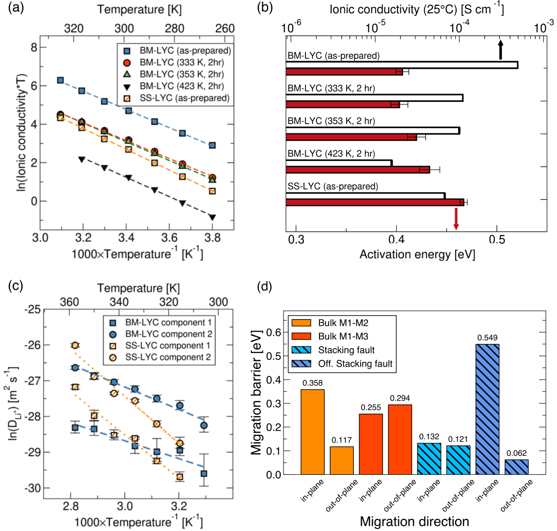
Figure 8: (a) Arrhenius behavior of EIS-measured ionic conductivity for as-prepared BM-LYC and heat treated samples (b) Room temperature ionic conductivity and activation energy for \text{Li}^+ long-range diffusion for various LYC samples (c) Variable temperature PFG-NMR measurements on as-prepared BM- and SS-LYC samples. All measurements were conducted at 7.05 T. (d) Predicted migration barriers in (eV) for \text{Li}^+ ions in different model structures: bulk M1 - M2 (orange bars), bulk M1 - M3 (red bars), stacking fault (light blue), and off-stoichiometric stacking fault (blue). The uncertainty of the migration barriers is \pm 0.06 eV. 65 All error estimates are for one standard deviation.
