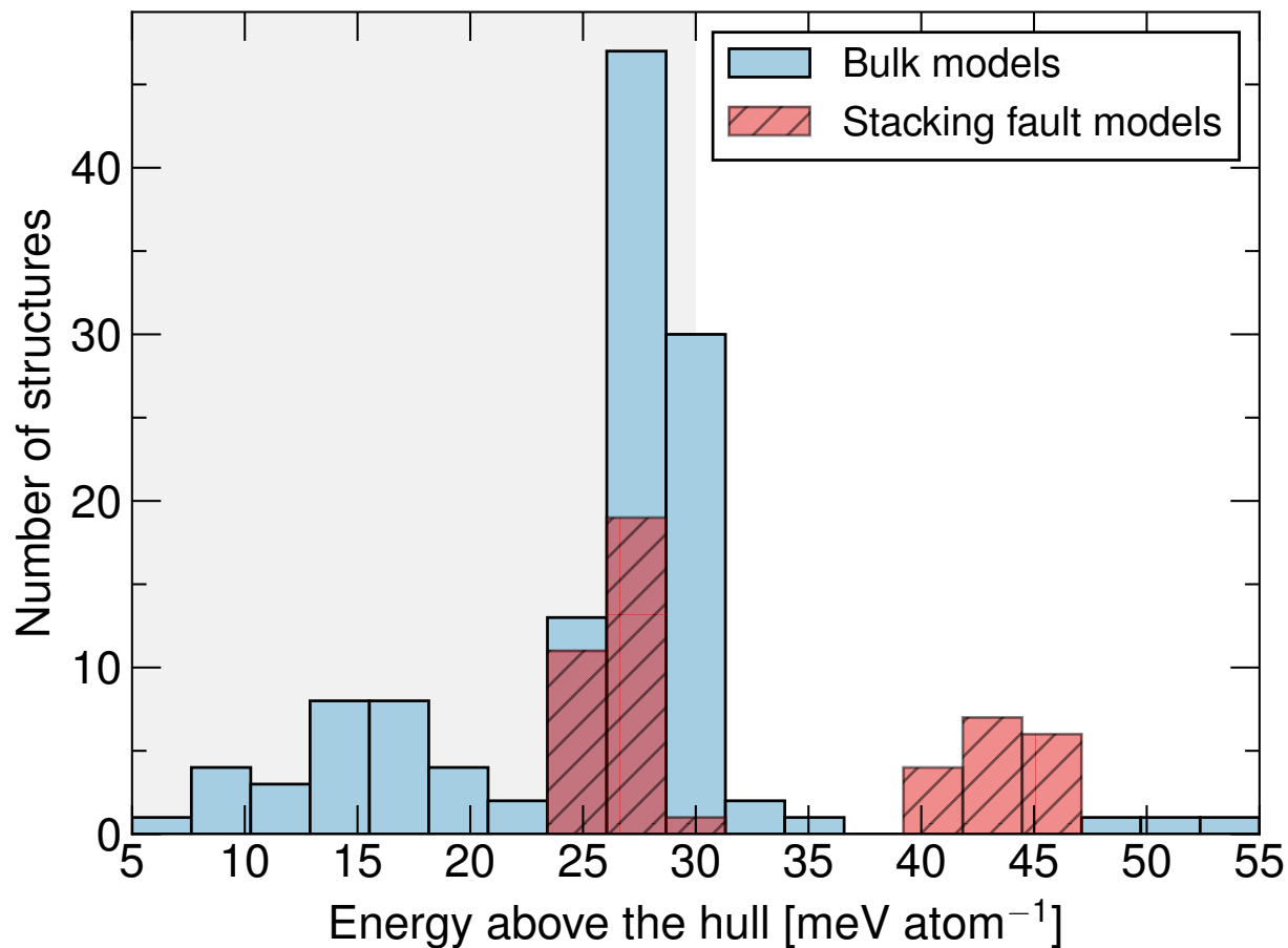
Figure 5: Distribution of predicted Li/Y orderings in \text{Li}_3\text{YCl}_6 vs. their relative thermodynamic stability, expressed as energy above the hull. Some of the 237 bulk orderings are shown with blue bars, whereas the 48 stacking faults by the red-hatched bars. Energetically accessible orderings below the 30 meV atom -1 threshold are enclosed in the gray shaded area. The figure displays only orderings up to 55 meV atom -1 .
