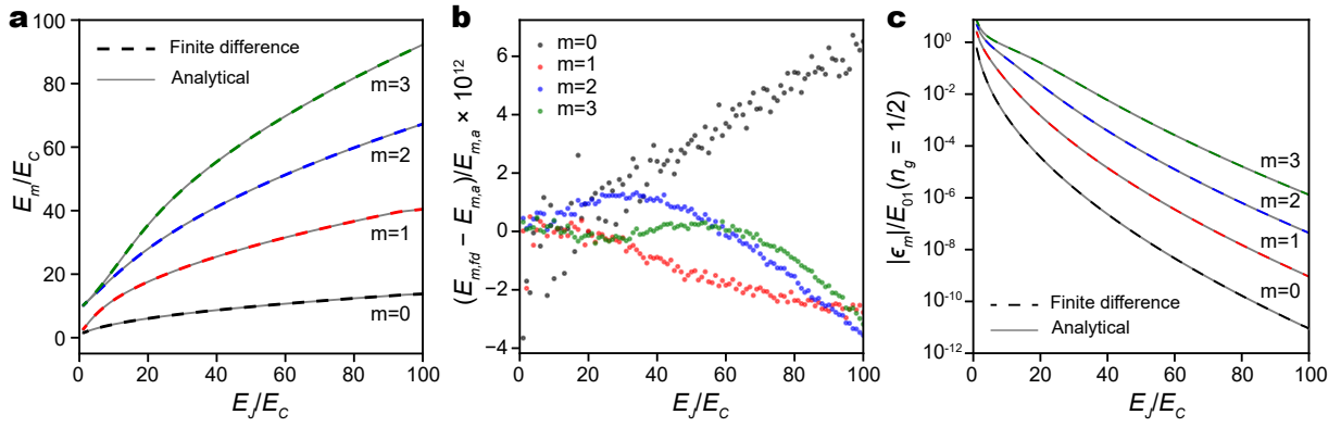
Figure C.1. (a) The first four eigenenergies of a SIS transmon, plotted versus E_J/E_C , for n_g = 1/2 , calculated using the analytical solutions (gray solid lines) and the finite difference method (dashed lines), as functions of E_J/E_C . (b) Relative errors of the finite difference solutions, calculated as (E_{m,fd} - E_{m,a})/E_{m,a} , in which E_{m,fd} and E_{m,a} are the m th eigenenergies given by the finite difference method and the analytical solution, respectively. (c) The charge dispersion \epsilon_m of the lowest four eigenstates of a SIS transmon (dashed lines), calculated by using the analytical solutions (gray solid lines) and the finite difference method (dashed lines), as functions of E_J/E_C .
