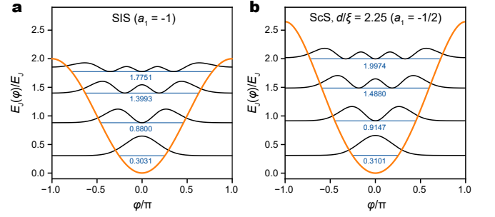
Figure 3. The eigenenergies (blue lines and numbers) and the probability densities ( |\Psi|^2 ) of the first 4 eigenstates of (a) a SIS transmon and (b) a nanobridge ScS transmon with d/\xi = 2.25 , both with E_J/E_C = 20 and n_g = 1/2 . The corresponding potential energies, normalized by E_J , are plotted in red lines for both transmons.
