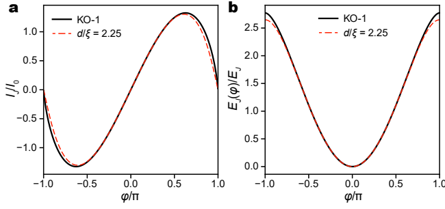
Figure B.1. (a) The CPR and (b) the potential energy E_J(\phi) of a KO-1 ScS junction at T = 0 K (black solid lines) are compared with the corresponding ones of a nanobridge ScS with d/\xi = 2.25 at the GL regime (red dashed lines).
