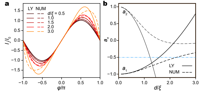
Figure A.1. (a) The CPRs of nanobridge junctions according to the closed form approximation by Likharev and Yakobson (LY, solid lines), compared with the numerical results (NUM, dashed lines). (b) The Maclaurin coefficients a_1 and a_2 , as functions of d/\xi , for LY solution and the numerical solution.
