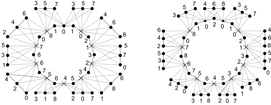
FIGURE 11. Optimal b -chromatic colorings of C_{10} \boxtimes P_3 and C_{11} \boxtimes P_3 .
