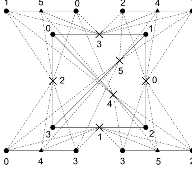
FIGURE 20. Optimal b -chromatic coloring of K_4 \square P_3 .
