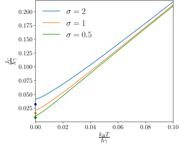
Figure 4. Critical coupling as a function of temperature for different choices of the variance \sigma of the Gaussian frequency distribution. The overdamped ratio is fixed \frac{m \gamma}{h} = 7 . The dots shown for k_B T = 0 represent \frac{J_C^cl}{h \gamma} for the noiseless model compatible with D = k_B T = 0 . The colors of the dots are related to the choice of \sigma as shown in the legend.
