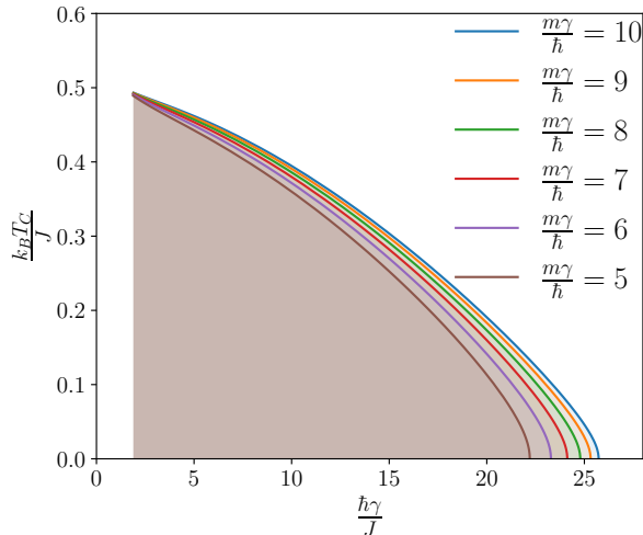
Figure 5. Phase diagram of the quantum model in the coupling-temperature space, where the coloured region indicates the synchronized phase. A quantum phase transition at zero temperature is apparent. The result is obtained for a Gaussian distribution of frequencies with zero mean and variance \sigma = 2 .
