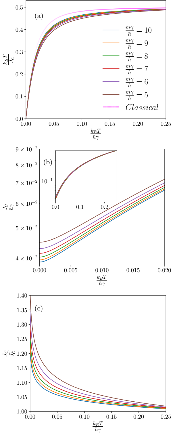
Figure 3. Temperature-dependence of the inverse of critical coupling in units of temperature (a) and (b) in logarithmic scale for different values of \frac{m \gamma}{h} . The legend in (a) holds for all the panels. In (a) the classical critical coupling (pink line) is plotted for reference for high temperatures. (c) Ratio between the quantum results and the classical one (extended to low temperatures) vs temperature. The difference in behaviour of the classical and quantum critical couplings is clearly evident close to zero temperature. All results are obtained for g(\omega) Gaussian with zero mean and \sigma = 2
