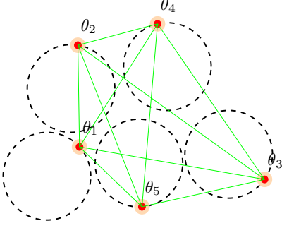
Figure 1. Representation of the classical Kuramoto model for N = 5 . A set of rotors (red dots on dashed circles) evolve with independent frequencies. Their mutual interactions (green lines) induce a phase transition to synchronised dynamics.
