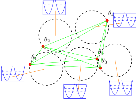
Figure 2. Representation of the quantum Kuramoto model. Same as Fig.1, with the rotors as quantum systems. The coupling to independent identical quantum baths is explicitly shown as an orange line connecting to a set of harmonic oscillators (blue boxes)
