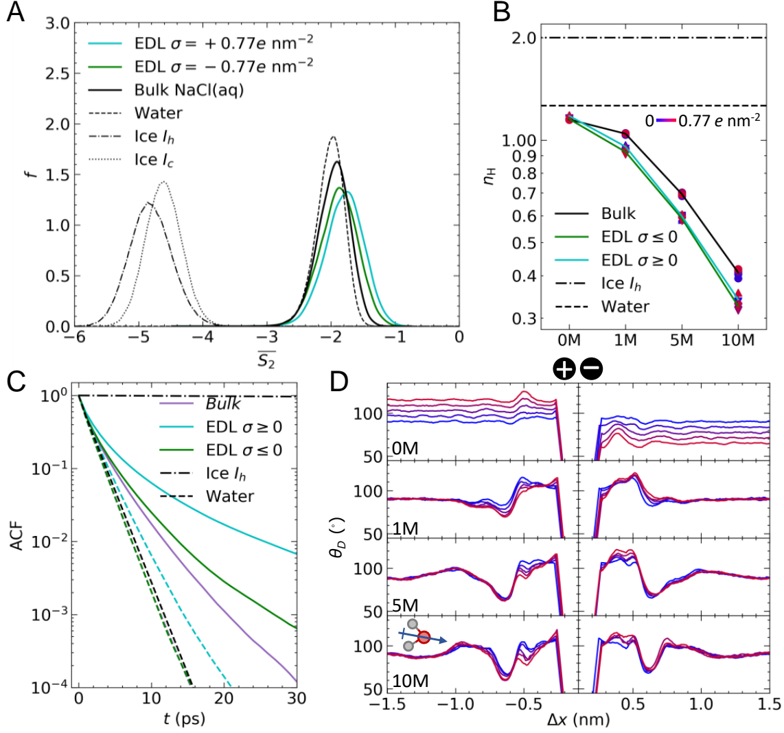
Figure 4: Water structure in the bulk and EDL regions of a CμMD simulation compared to pure water (Water) and hexagonal ice ( I_h ). A) Water local average approximate pair entropy ( \overline{S_2} ) calculated for 5M NaCl(aq) at graphite with charge density, |\sigma| = 0.77e \text{ nm}^{-2} . B) Number of donated hydrogen bonds per water molecule ( n_H ). Colours blue→red indicate increasing solution charge density as shown by the scale inset. Solid lines show the mean n_H values at each concentration for water in the bulk (circles), negatively (inverted triangles) and positively (triangles) charge interface regions. Uncertainties in the data are on the scale of the size of data points. C) H-bond lifetimes, as indicated by the time-dependent H-bond autocorrelation function (ACF). Data are provided for the case where |\sigma| = 0.77e \text{ nm}^{-2} and ion concentrations are 0M (dashed lines; the curves for bulk and EDL \sigma \leq 0 are nearly perfectly overlaid on the graph) and 10 M (solid lines). D) Water molecule orientation as indicated by the average angle between the water molecule dipole moment (shown by the arrow on the water molecule inset) and the normal to the carbon basal surface ( \theta_D ). The colours indicate surface charge density (see the scale in B). The data in D were smoothed using a zero th -order Savitsky-Golay filter with a 0.05 nm window size.
