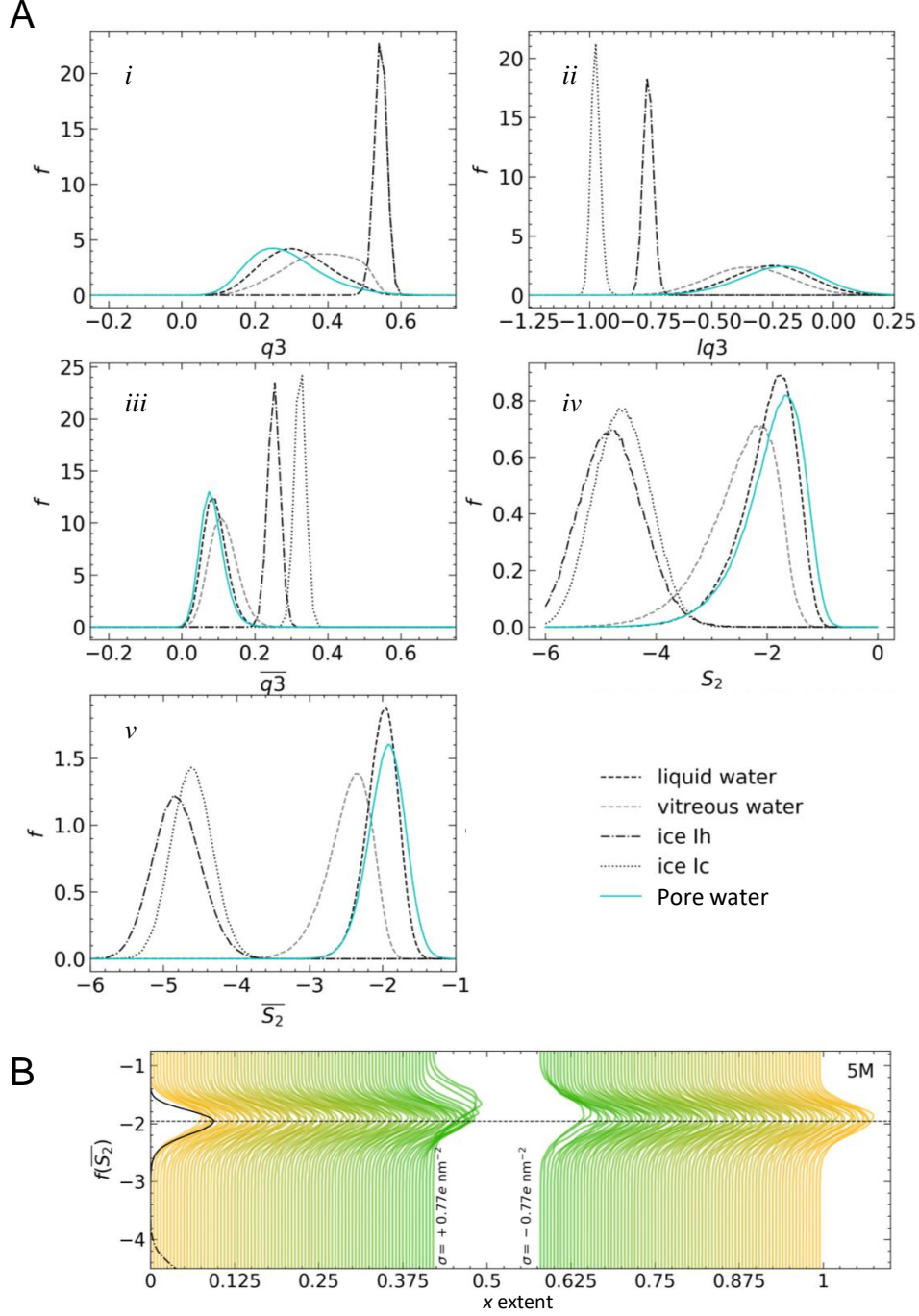
Figure S6: A) Order parameter analysis for water in CμMD simulations of 5 M NaCl(aq) at charged graphite with surface charge density, |\sigma| = 0.77 e \text{ nm}^{-2} . The probability density for q3 ( i ), local q3 ( ii ; lq3 ), local average q3 ( iii ; \overline{q3} ), approximate pair entropy ( iv ; S_2 ) and local average approximate pair entropy ( v ; \overline{S_2} ) are provided. The distributions for water in bulk liquid, vitreous (liquid water crash cooled to 100 K), hexagonal ice (ice I_h ) and cubic ice ( I_c ) are also provided. B) Probability densities for \overline{S_2} in slices of the cell x axis. The bulk liquid water and ice I_h distributions are provided on the y -axis.
