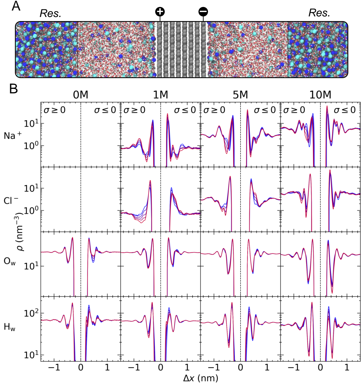
Figure 1: A) Snapshot from a C\mu\text{MD} simulation of \text{NaCl}(\text{aq}) at charged graphite projected onto cell x and y axes. The dashed lines indicate the edge of the reservoir ( Res. ); grey, blue, cyan, red and white spheres indicate C, \text{Na}^+ , \text{Cl}^- , O and H atoms, respectively. B) Mean solution atom densities, \rho , determined as a function of distance from the graphite electrode, \Delta x , for a range of target bulk solution ion concentrations. The solution concentration and atom type are indicated at the top and left of the grid. Colours blue→red indicate increasing solution charge densities from |\sigma| = 0 \rightarrow 0.77 \text{ e nm}^{-2} .
