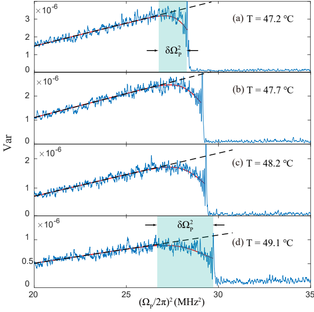
Figure 5. Variance measured at different temperatures. We measured the different variance characteristics at temperatures of (a) T=47.2^\circ\text{C} , (b) T=47.7^\circ\text{C} , (c) T=48.2^\circ\text{C} , and (d) T=49.1^\circ\text{C} . The results show that as the temperature increases, the divergence of the variance from the linear regime becomes more obvious. The early warning signal regimes shown in (a) and (d) are marked as the blue shaded areas for comparison. The solid red lines are the fittings with the function y = p(x - 20)e^{q(x-20)^\alpha} + s , where \alpha = 16.46 \pm 0.22 for T=47.2^\circ\text{C} , \alpha = 12.69 \pm 0.10 for T=47.7^\circ\text{C} , \alpha = 10.89 \pm 0.07 for T=48.2^\circ\text{C} , and \alpha = 8.59 \pm 0.07 for T=49.2^\circ\text{C} .
