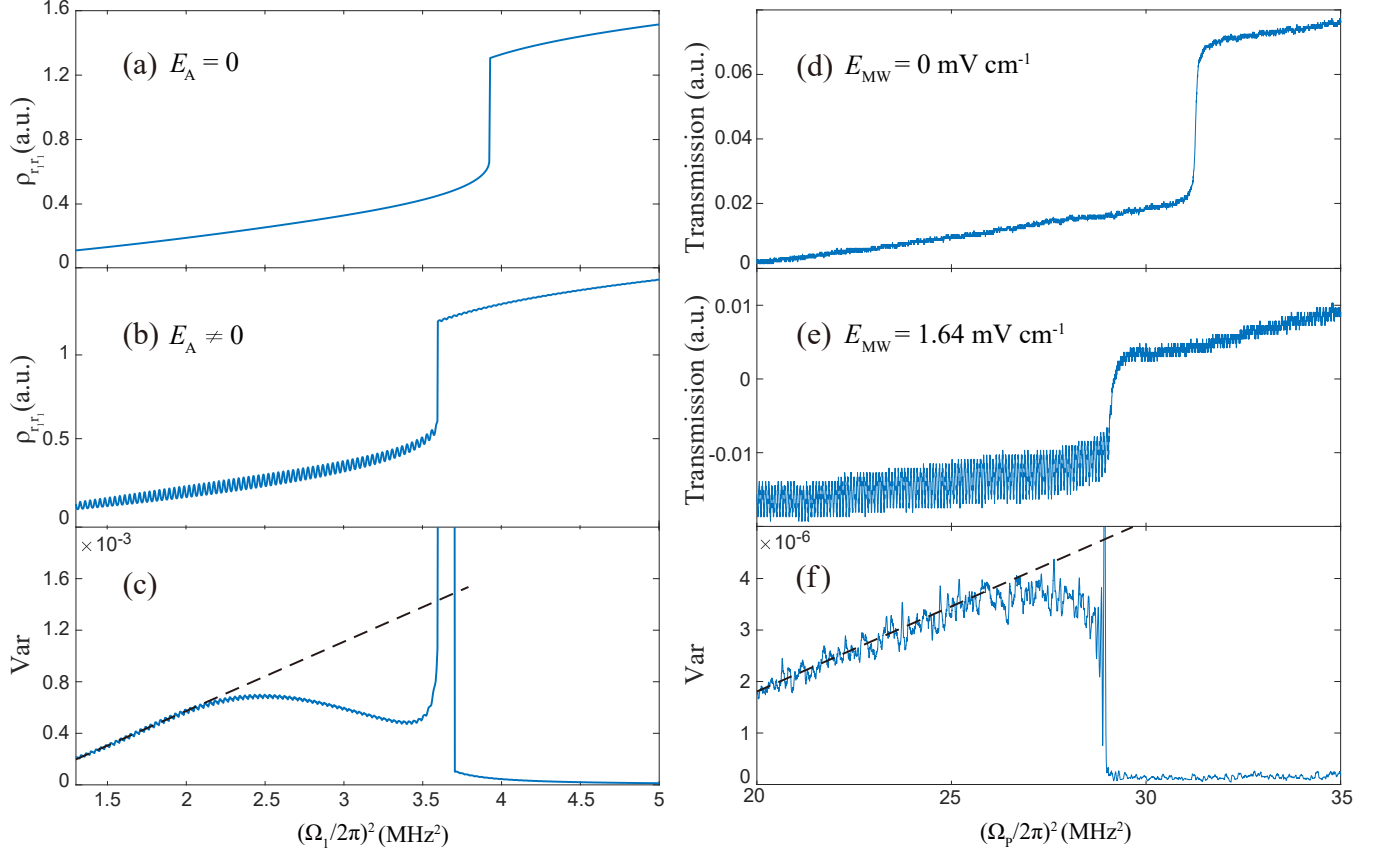
Figure 2. Theoretical and experimental results without and with the driving MW field. (a), (b) Theoretical simulations of the population \rho_{r_1 r_1} of the Rydberg atoms with different electric field amplitudes: (a) E_A = 0 mV/cm and (b) E_A \neq 0 mV/cm. (c) Variance calculated from (b). (d), (e) Experimental transmission spectra under the different MW field amplitudes: (d) E_{\text{MW}} = 0 mV/cm and (e) E_{\text{MW}} = 1.64 mV/cm. In this case, the scanning period T_s = 1 ms. (f) Measured variance from (e).
