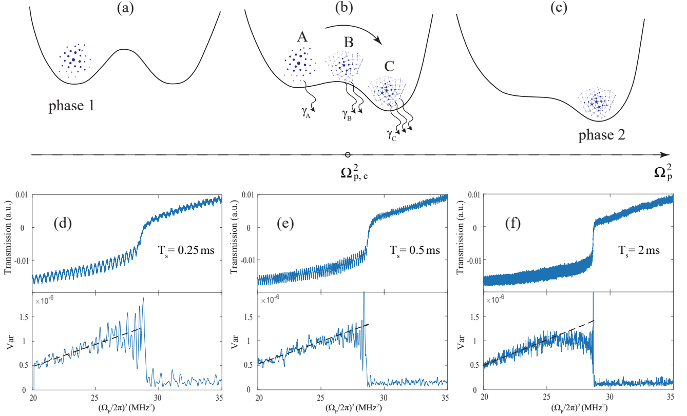
Figure 3. Time evolution of the system during the phase transition process. (a)-(c) Double well model used to describe the phase transition and the critical slowing down phenomenon. With increasing \Omega_p^2 , the system is initially in phase 1 ( \Omega_p^2 < \Omega_{p,c}^2 , where \Omega_{p,c}^2 is the tipping point), and it then evolves from state A to state B when close to the tipping point, before finally making the transition to phase 2 ( \Omega_p^2 > \Omega_{p,c}^2 , state C). In this process, the system states A, B, and C have different interaction-induced dissipations \gamma_A , \gamma_B , and \gamma_C , respectively, where \gamma_C > \gamma_B > \gamma_A . (d)-(f) Measured transmission spectra and their corresponding variances within scanning times of (d) 0.25 ms, (e) 0.5 ms, and (f) 2 ms.
