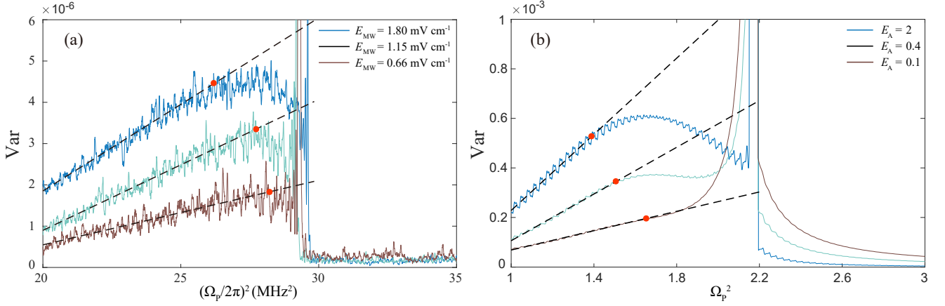
Figure 4. Trend of variance at different MW field intensities. (a) Variance measured at the different MW field intensities of E_{\text{MW}}=1.80 mV/cm (blue), E_{\text{MW}}=1.15 mV/cm (light green), and E_{\text{MW}}=0.66 mV/cm (brown); see the Methods section for further details. To provide a better comparison of the signals at the different microwave intensities, we normalized the variance of the transmission for easier reading. The variance at 0.66 mV/cm is amplified by a factor of four and the variance at 1.15 mV/cm is amplified by a factor of 1.5, but the variance at 1.80 mV/cm is not amplified. (b) Theoretical simulations at the different modulation strengths of E_A = 2 (blue), E_A = 0.4 (black), and E_A = 0.1 (brown), where we normalized the simulated results using an amplification factor of 10 at E_A = 0.4 and an amplification factor of 20 at E_A = 0.1 ; the variance at E_A = 2 was not amplified. The red points correspond to the points where the variance diverged from the linear function in each case. In these processes, the tipping points for the different MW field intensities are calibrated to be in the same position for ease of comparison by slightly adjusting the coupling detuning.
