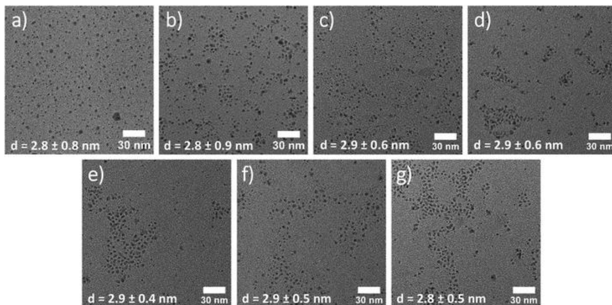
Fig. 2 TEM images of (a) Ag 2 S QDs before and during the cation exchange at (b) 5 min, (c) 15 min, (d) 30 min, (e) 50 min, (f) 80 min, and (g) 120 min of reaction time. Scale bar 30 nm (bottom right) and average QD size and standard deviation (bottom left) for each image.
