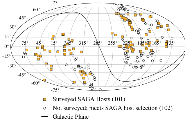
Figure 2. Sky distribution of 203 SAGA Milky Way analog systems as defined in Section 2.2. Orange squares show the 101 systems that have been surveyed and are presented in this work. Empty circles show systems that match our host selection (i.e., from the “Grand List” with criteria 1a through 1g applied) but have not been surveyed.
