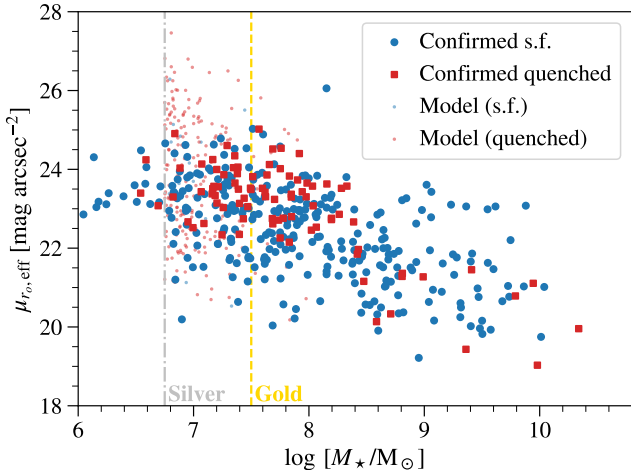
Figure 10. The effective surface brightness–mass distribution of confirmed SAGA satellites; the large blue circles and large red squares show star-forming and quenched satellites, respectively. The small dots show a random realization of satellites that we may have missed in the Gold and Silver samples, according to our incompleteness model; the color of the small dots indicates whether the missed satellites are star forming (blue) or quenched (red). The gold and silver vertical lines show the corresponding stellar mass limit of the Gold and Silver samples.
