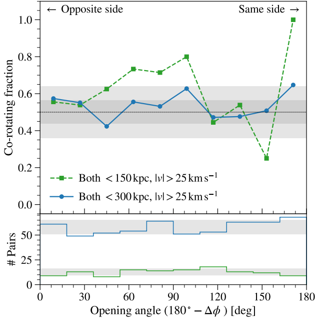
Figure 17. Upper: Fraction of corotating satellite pairs in bins of opening angles between the pairs. We follow the convention of (Phillips et al. 2015), such that a pair of satellites on opposite sides of a host have an opening angle of 0^\circ . The green squares show the corotating fraction from pairs of satellites that are within 150 kpc of their hosts. The blue points show the same but including all confirmed satellites up to 300 kpc from their hosts. The dark and light gray bands show the 1\sigma and 2\sigma of co-rotation fraction when all satellites are assigned a position angle (relative to their hosts) uniformly at random. Lower: The number of pairs in bins of opening angles. Same as above, green and blue lines indicate satellites that are within 150 and 300 kpc, respectively. The gray bands show the 1\sigma distribution of the number of pairs when all satellites are assigned a position angle (relative to their hosts) uniformly at random. See Section 5.8 for details about how the corotating fraction is calculated.
