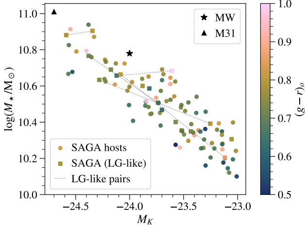
Figure 3. Distribution of the K -band absolute magnitudes (x-axis, Jarrett et al. 2000), stellar masses (y-axis), and g-r colors (color of the markers) of 101 SAGA host galaxies. The circle and square markers indicate regular and Local Group-like hosts, respectively (here “Local Group-like” means having exactly one MW-mass companion within 1 Mpc). Square markers that are connected by a thin dotted line are Local Group-like pairs. The black star and triangle show the luminosities and stellar masses of the Milky Way and M31, respectively.
