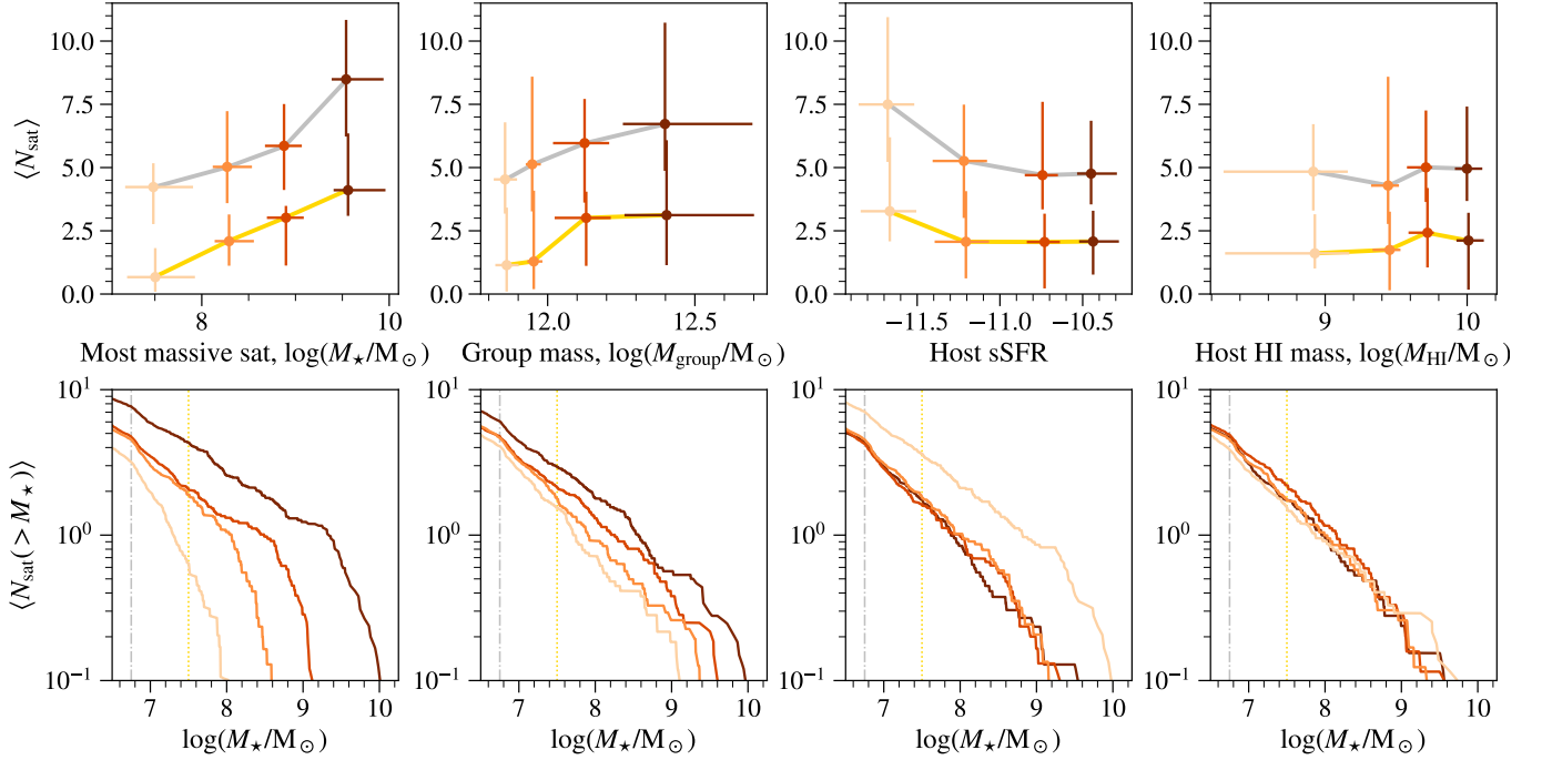
Figure A.3. How SAGA satellite systems vary across host/system properties. The upper panels are the average number of satellites per system, and the lower panels are satellite stellar mass functions. The SAGA systems are split into quartiles using four different host/system properties: (from left to right) the stellar mass of the most massive satellite, the group (halo) mass, the specific star formation rate of the host galaxy, and the HI mass of the host galaxy. Each panel in the upper row shows the average number of satellites per system as a function of the corresponding host/system property. The points connected by the gold line (lower line) show the average number of satellites in the Gold sample, and the higher points connected by the silver line (upper line) show that of the Gold+Silver sample. Each panel in the lower row shows how the average cumulative stellar mass function changes with the corresponding host/system property. The colors of the points in the upper panel correspond to the colors of the lines in the lower panel, with darker colors indicating higher quartiles.
