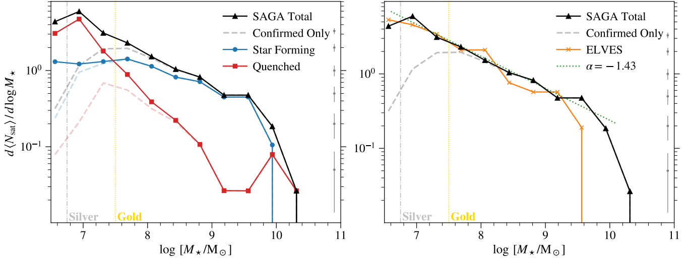
Figure 9. Left: The average satellite stellar mass function (SMF) of 101 SAGA systems, shown in the differential form ( d\langle N_{\text{sat}} \rangle / d \log M_* ). The darker solid curves show the SMF when survey incompleteness is taken into account, while the fainter dashed curves show only confirmed satellites. The curves with black triangles, blue circles, and red squares show all satellites, only star-forming satellites, and only quenched satellites, respectively. The gold dotted and silver dot-dashed vertical lines show the corresponding stellar mass limits of the Gold and Silver samples. These SMF data points are provided in Table C.5. Right: Same as the left panel, but comparing the SAGA satellite SMF with the ELVES Survey (orange crosses) and a constant slope of -0.43 (typically quoted as \alpha = -1.43 ; green dotted line). Note that the SAGA total SMF (solid black line) has been corrected for incompleteness, while the ELVES SMF shown here has not. The error bars near the right border of both panels show the Poisson error on the SAGA SMF.
