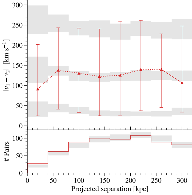
Figure A.5. Upper: The velocity difference between all pairs of confirmed satellites in the SAGA Survey, binned by projected separation between the two satellites. In each bin, the distribution of the velocity difference is shown as the median value (red triangles) and the 16th and 84th percentiles (lower and higher caps). The light gray bands show the 1\sigma distribution of the velocity difference when all satellites are assigned a position angle (relative to their hosts) uniformly at random. Lower: The number of pairs in bins of projected separation. The observed numbers are shown in red lines. The gray bands show the 1\sigma distribution of the number of pairs when all satellites are assigned a position angle (relative to their hosts) uniformly at random.
