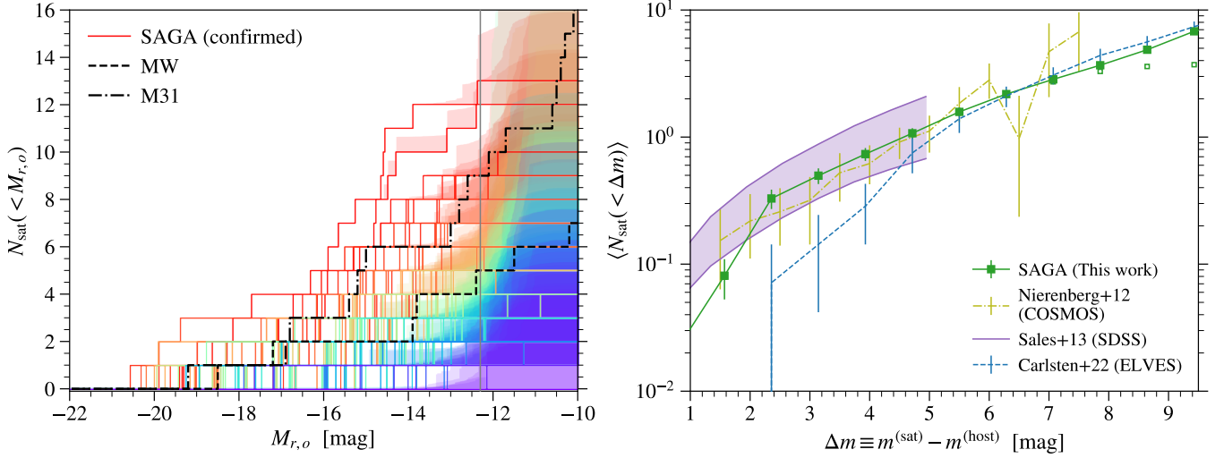
Figure A.2. Reproduction of Figure 12 (satellite luminosity functions) of Paper II from DR2 with the DR3 SAGA data. Left: Cumulative satellite r -band luminosity function for each of the 101 SAGA systems (colored solid lines), MW (black dashed line), and M31 (black dot-dashed line). The colored solid lines show only the confirmed SAGA satellites, and the shaded region shows incompleteness correction as discussed in Section B.1. The SAGA Survey’s designed depth is about M_{r,o} = -12. , shown as the vertical gray line. Right: Average cumulative satellite r -band luminosity function, with satellite luminosity normalized by the luminosities of their respective host galaxies (calculated as differences in magnitudes). The average luminosity function of SAGA systems is shown as the green filled squares. The incompleteness correction is included in the filled squares, and uncorrected results are shown as green open squares. The yellow dot-dashed line shows the average luminosity function of systems in the COSMOS field (Nierenberg et al. 2012), the purple band SDSS (Sales et al. 2013), and the blue dashed line the ELVES Survey (Carlsten et al. 2022). See text in Appendix A for the specific system selections. The error bars show Poisson noise on the luminosity functions.
