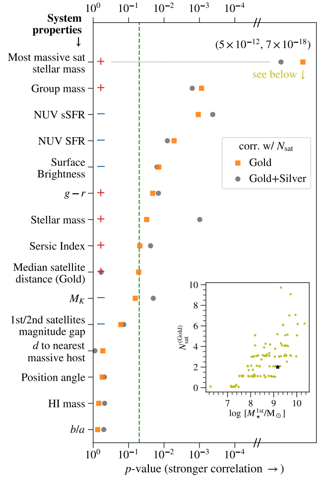
Figure 15. The correlation strength (shown as p -values) between each host property shown on the y-axis and the number of satellites per host in the Gold (shown as orange squares) and Gold + Silver (shown as gray circles) samples, presented as p -values from the Spearman rank correlation test. The plus and minus signs on the left show the sign of the correlation. The vertical line indicates a p -value of 0.05 (corresponding to a correlation coefficient of 0.2 with 101 systems). The p -values for the correlation between the most massive satellite mass and the numbers of satellites in both samples are extremely low, and are not shown to scale. The inset shows a scatter plot between the most massive satellite mass and the number of satellites in the Gold sample to demonstrate the observed correlation; the black star in the inset shows where the MW system would be located in this plot. See Section 5.7 for a more thorough discussion of the host properties’ meaning.
