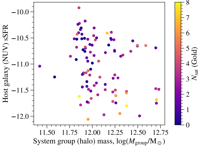
Figure A.4. Same as Figure 16 but the y-axis here shows the host galaxy's sSFR (inferred from NUV measurements; values shown are \log[M_\star/M_\star \cdot \text{yr}] ).
