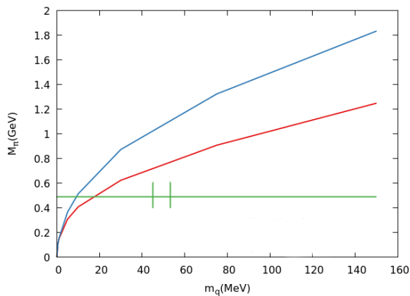
FIG. 14: The Gell-Mann-Oakes-Renner relation for the pseudoscalar mesons over the ground-state BCS vacuum. The curves ascend too quickly. (The lower one is obtained from the calculated mass spectrum M(m) and the upper one from the GMOR relation from our computed f_\pi and regularized condensate, they converge at low quark mass). The green marks show the experimental value of the Kaon K^- mass and the flavor-averaged quark mass interval m_q \in (90, 107) MeV, obtained from tabulated strange and light quark masses at a scale of 2 GeV. Ideally, the curves would have passed through that interval, but f_\pi in the model is too small.
